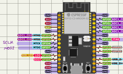
ESP32-C3-DevKitC-02
